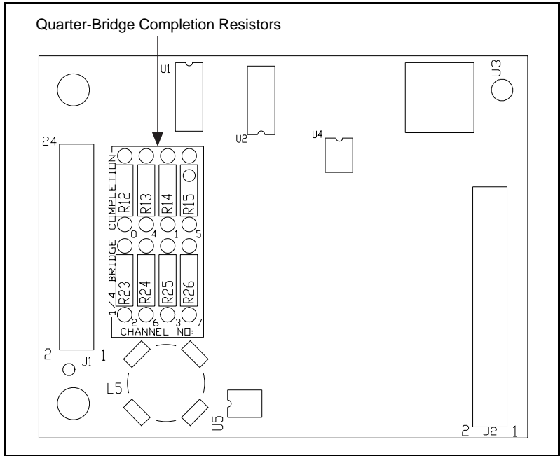
Figure 3-2. Quarter-Bridge Completion Resistors
